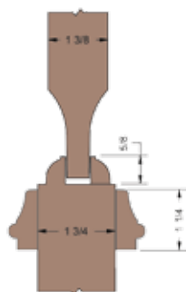
Recessed Molding WB31 Bolection Standard Panel
