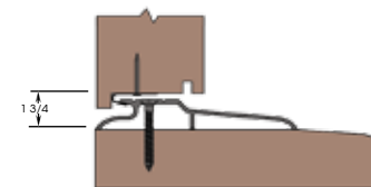
Interlocking Sill
