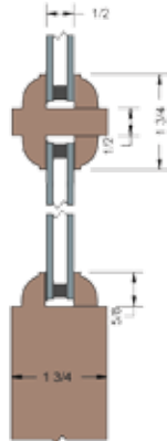
Recessed Molding & 1 3/4" TDL Bar
