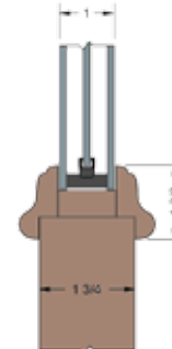
Raised Molding 1" I.G.
