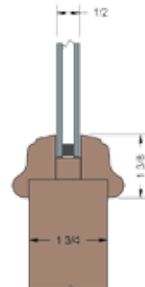
Raised Molding 1/2" I.G.
