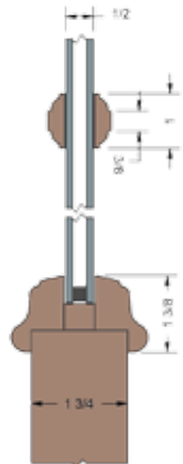
Raised Molding & 1" SDL Bar
