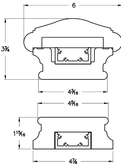
Nautilus RS10600 Works with 3-1/2" Baluster or Smaller
