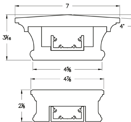
Nautilus RS20700 Works with 3-1/2" Baluster or Smaller
