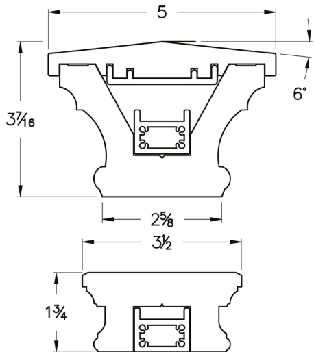
Nautilus RS20500 Works with 2-1/2" Baluster or Smaller
