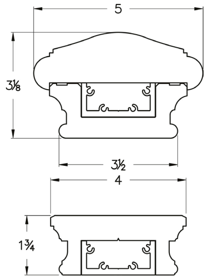
Nautilus RS10500 Works with 2-1/2" Baluster or Smaller
