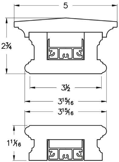
Nautilus RS50500 Available in Gooseneck; Works with 2-1/2" Baluster or Smaller
