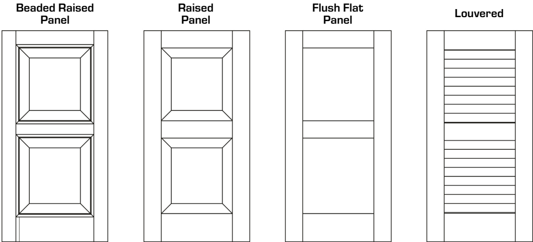
The rear detail of Beaded Raised Panel and Raised Panel is the same as the front of Flush Flat Panel.
