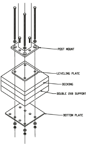
NEWELMOUNT-W POST MOUNT HARDWARE KIT FOR WOOD APPLICATION
