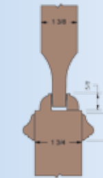
Recessed Molding WB11 Bolection Standard Panel
