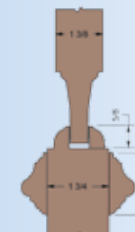
Recessed Molding W/ WB21 Bolection Classical Panel
